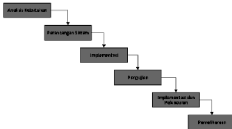
Gambar 1 Metode waterfall
