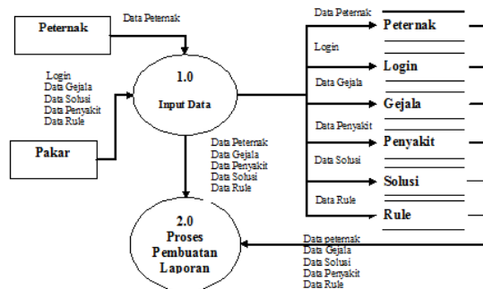
Gambar 3.2 Diagram Level 0
