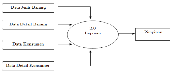
Gambar 3.6. Diagram Level 2
