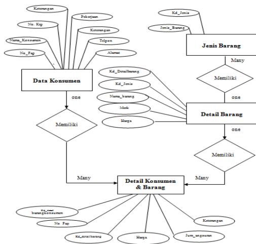
Gambar 3.7. Entity Relationship Diagram
