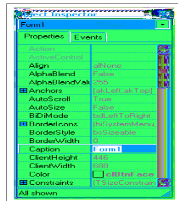
Gambar 7. Object Inspector
