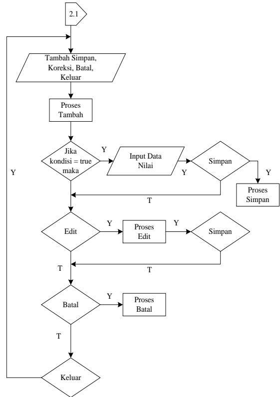
Gambar 21 Flowchart Penilaian
