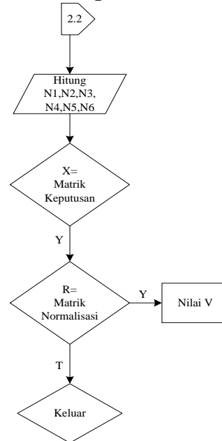
Gambar 21 Flowchart Penilaian
