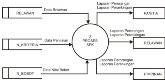
Gambar 8. Diagram Detail Level 2
