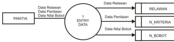
Gambar 7. Diagram Detail Level 1
