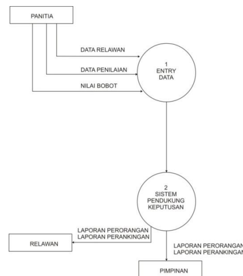
Gambar 6. Diagram Level 0
