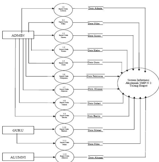
Gambar 4. Data Flow Diagram Level 1 Proses Maintenance Data
