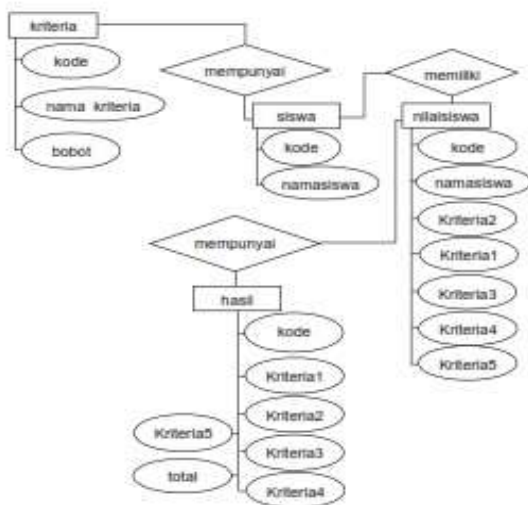
Gambar 3.5 Diagram ERD
