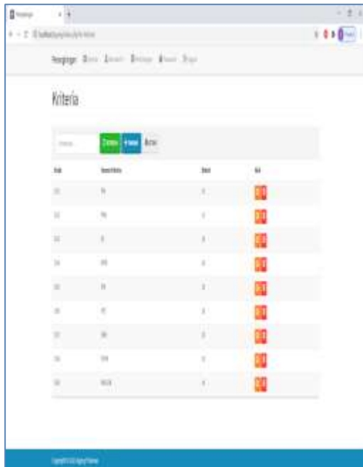
Gambar 4.3 Tampilan Kriteria
