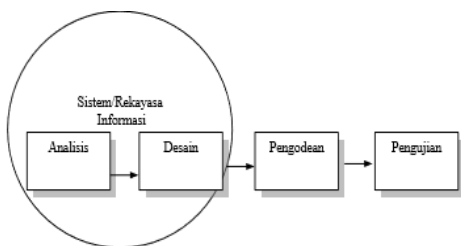
Gambar 3.1 Incremental System
