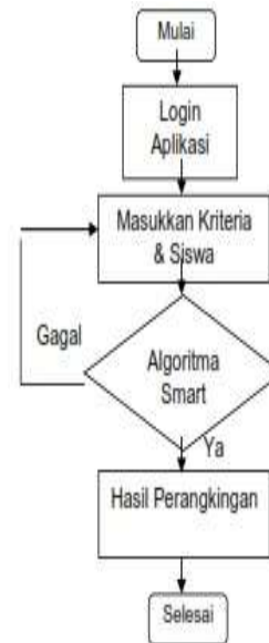
Gambar 3.2 Flowchart
