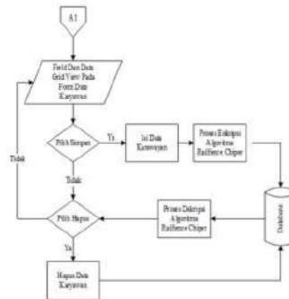
Gambar flowchat .5 flowchart input data karyawan
