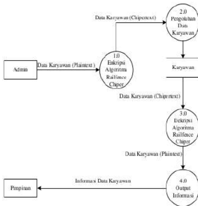
Gambar 8 Diagram Level 0
