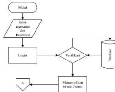
Gambar 3 flowchart login
