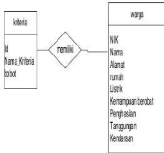
Gambar 6 ERD (Entity Relationship Diagram)
