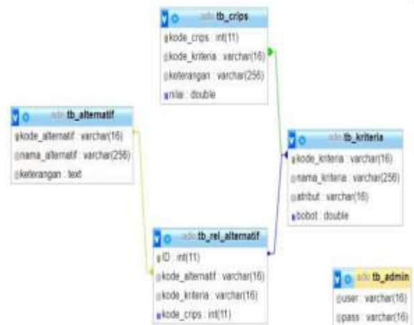
Gambar 3.4 Diagram ERD
