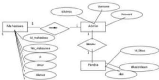
Gambar 3.5 Entity Relationship Diagram (ERD)
