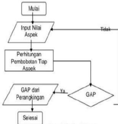
Gambar 3.4 Flowchart Algoritma
