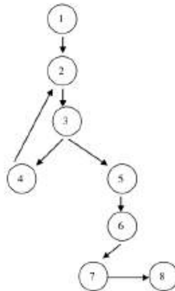
Gambar 19 Graph Whitebox
