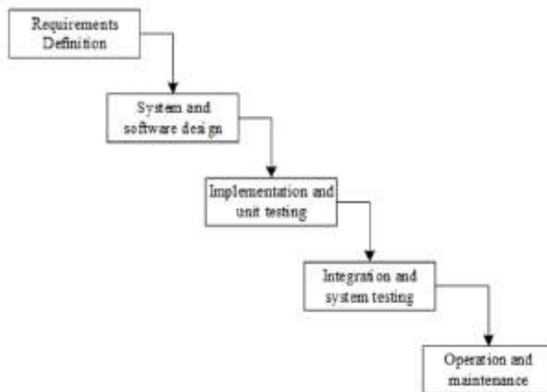
Gambar 1 Metode Waterfall
