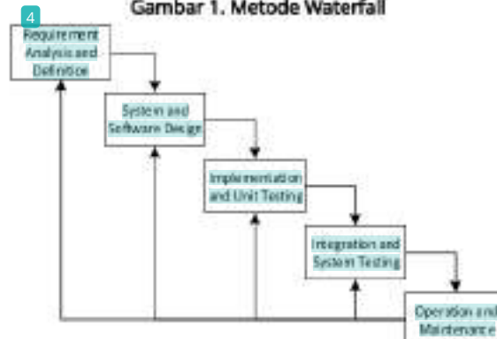
Gambar 1. Metode Waterfall
