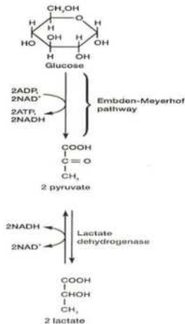
Figure 3. Metabolic pathway homofermentative lactic acid (Huda, 2012)
